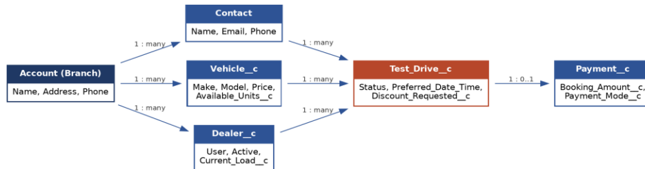
Figure 2: Entity-relationship diagram for the Vision Motors data model
