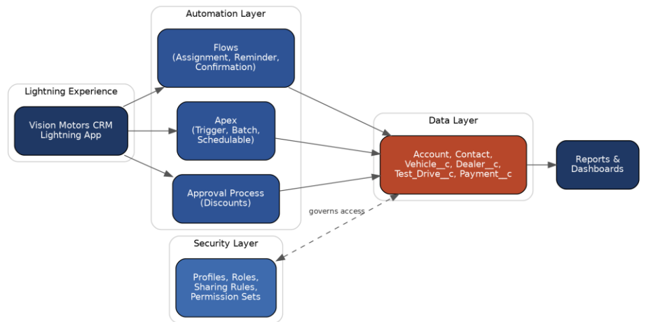
Figure 1: Vision Motors CRM – solution architecture overview
